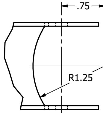
DETAIL B
